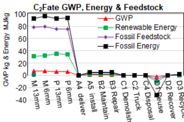
Figure 5 GWP A1 to D3/kg Functional Unit
